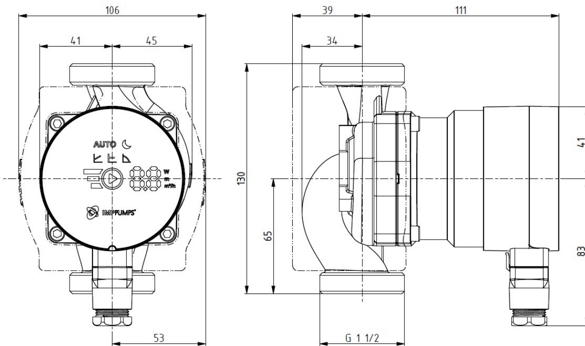
Dimension drawing
